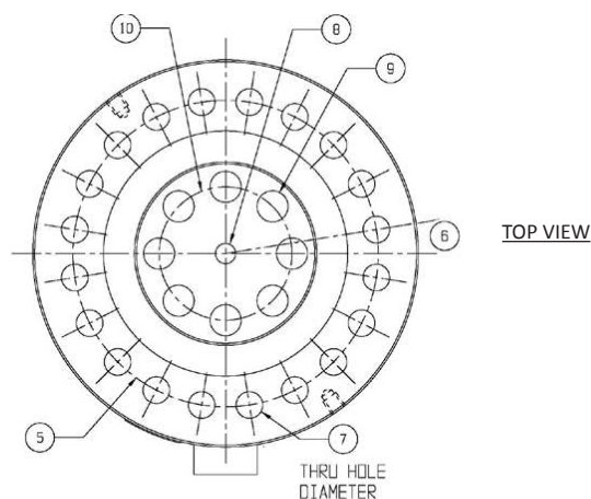
Model 1228ACK-50K (shown)
